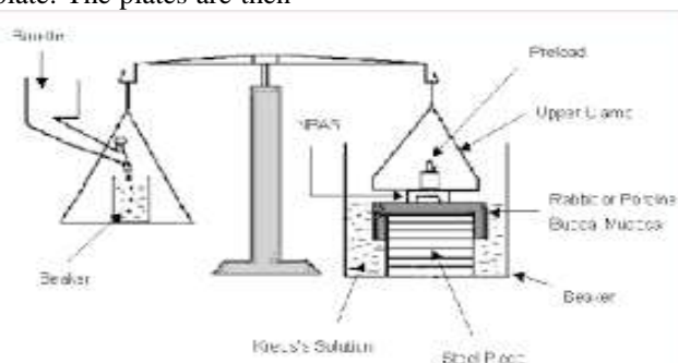
FIGURE 2: MEASUREMENT OF MUCOADHESIVE STRENGTH
