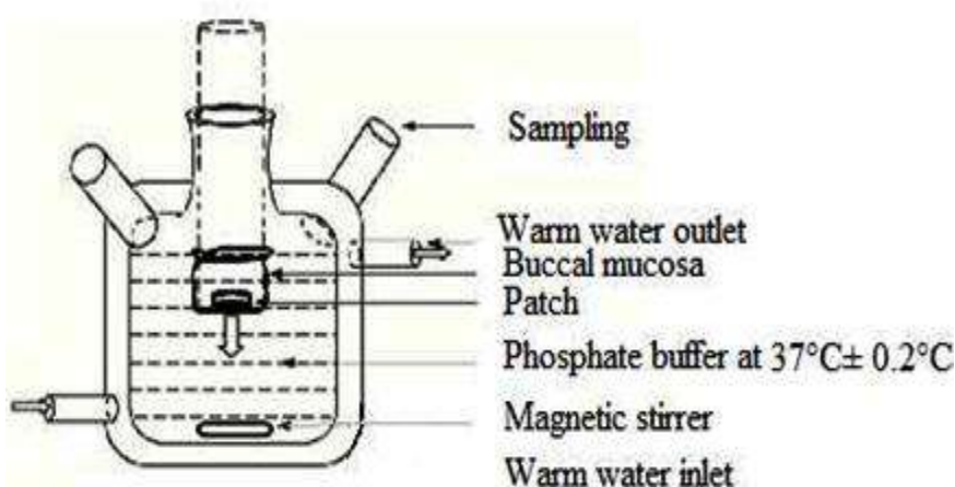
FIGURE 3: SCHEMATIC DIAGRAM OF FRANZ DIFFUSION CELL FOR BUCCAL PATCH
